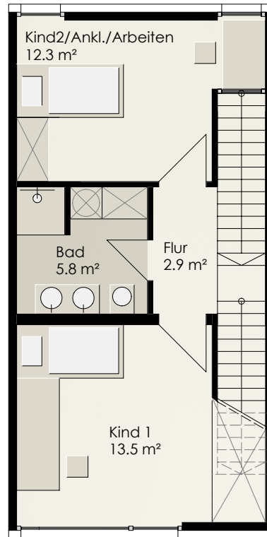
Grundriss OG, V5.2, 10 m
