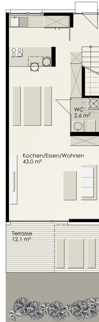
Grundriss EG, V7, 11m
