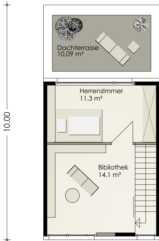
Grundriss DG, V6, 10m
