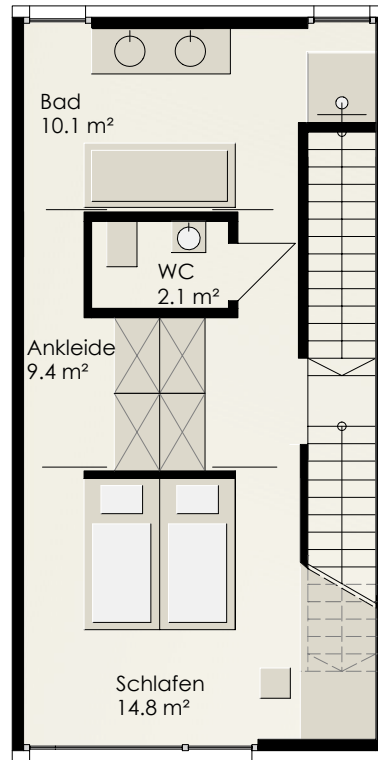
Grundriss OG, V6, 10m
