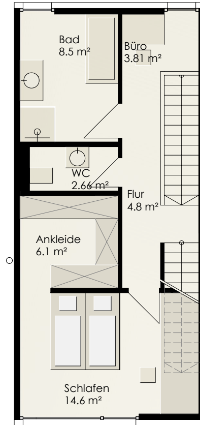
Grundriss OG, V4.3, 11 m
